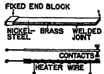
Bimetallic strip used as a time-delay switch.
